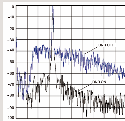
Digital Noise Reduction Performance
