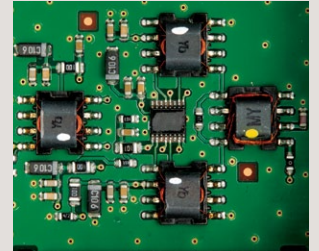
Mixer Unit
